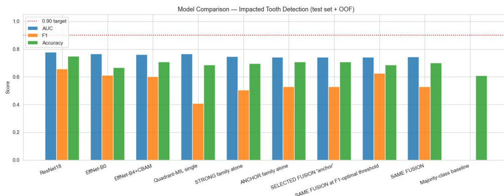
Figure 4.2: Executed model-comparison summary. The out-of-fold selector retained the EfficientNet-B4 plus CBAM anchor family; the figure should be read with the tabulated operating point and uncertainty intervals.
